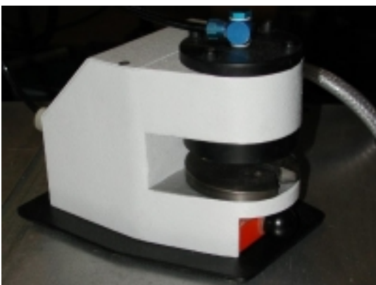
Lenz Pneumatic Depinner
